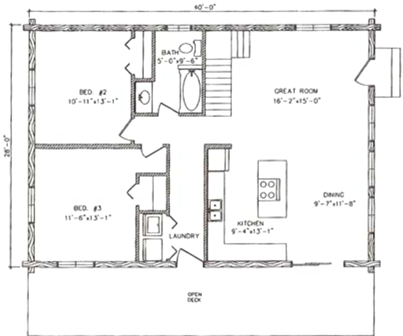
LARK MAIN FLOOR PLAN 1120 SQUARE FEET 1805 SQ. FT. TOTAL
